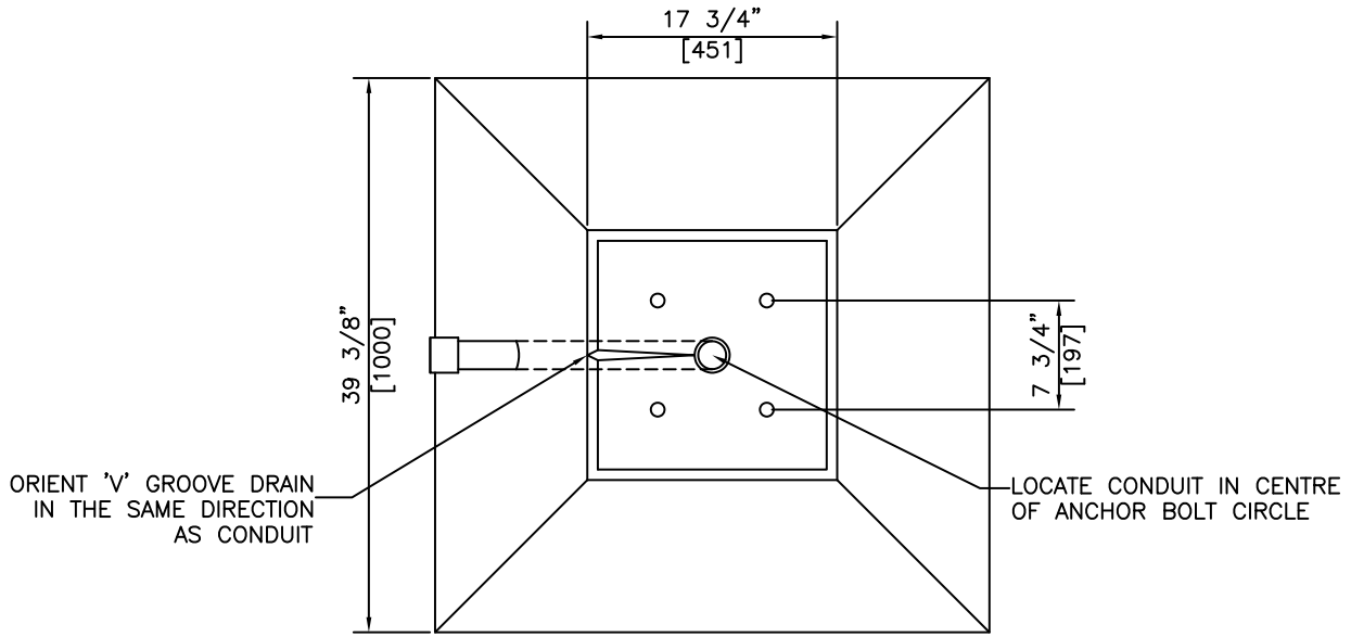
PLAN
