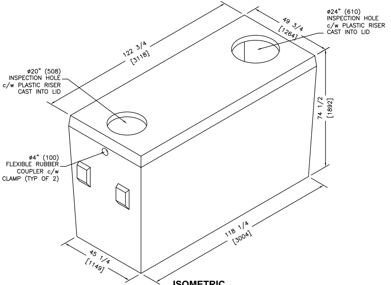
ISOMETRIC
